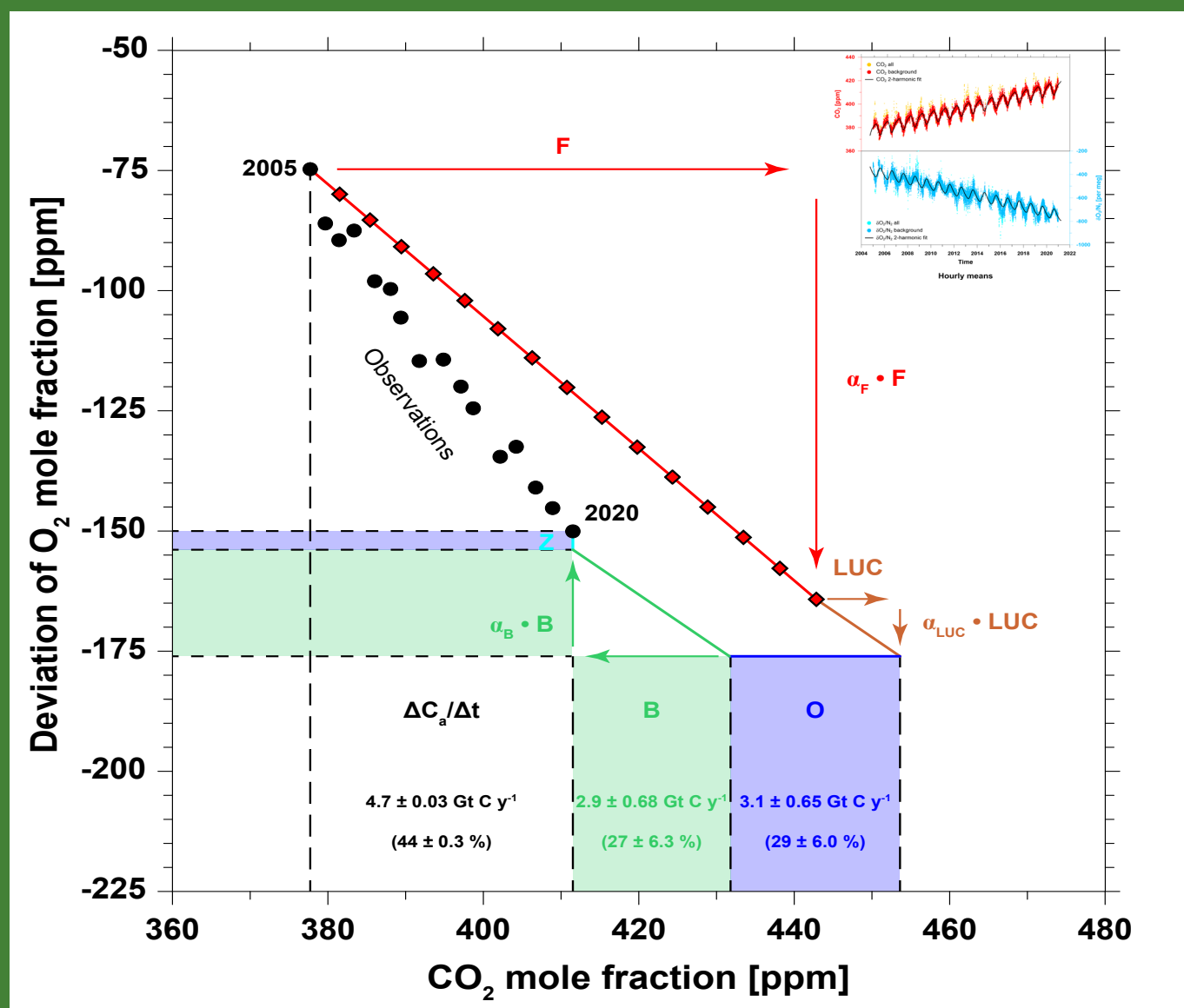
Figure 2. Analysis of the global carbon budget based on observations of CO 2 and O 2 at WMO GAW global station Jungfraujoch, Switzerland [7]. The top-right insert shows the underlying hourly time series for CO 2 and the O 2 /N 2 ratio from 2005 to 2021. The outcome of the analysis shows that over the 16-year period the percentage of emissions remaining in the atmosphere is 44% ( \Delta C_a/\Delta t = 0.44 ), global biosphere uptake (B) is 27% and global ocean uptake (O) is 29%. The red line depicts the theoretical changes in CO 2 and O 2 levels in response to fossil fuel emissions (F) and emission associated with land-use change (LUC). (Z) shows changes in O 2 level due to ocean thermal outgassing.
