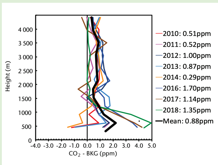
Figure 12. Annual mean vertical profiles at ALF aircraft measurement site in Brazil [28].
