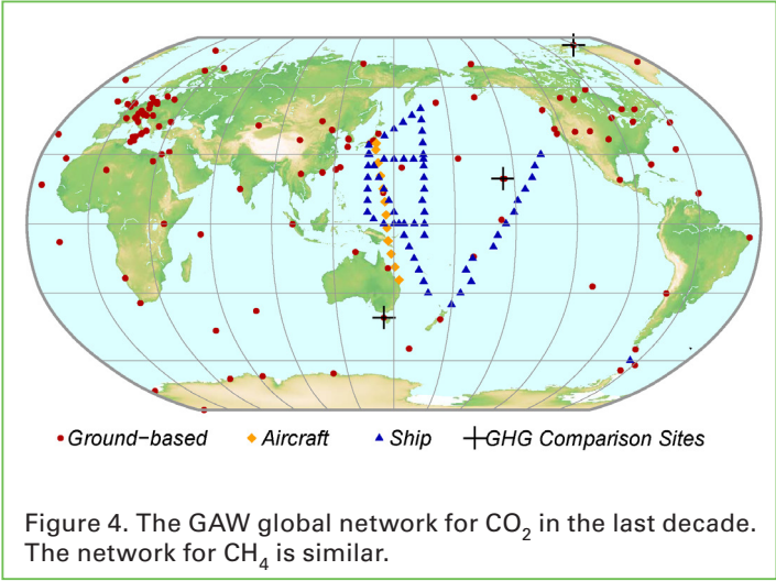
The WMO GAW Programme coordinates systematic observations and analyses of GHGs and other trace species. Sites where GHGs have been measured in the last decade are shown in Figure 4. Measurement data are reported by participating countries and archived and distributed by the WMO World Data Centre for Greenhouse Gases (WDCGG) at the Japan Meteorological Agency.
