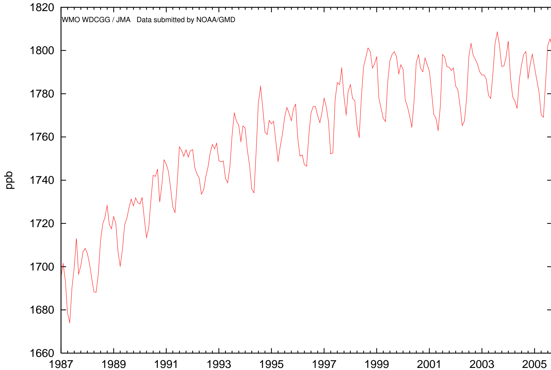
Mauna Loa 19.539N, 155.578W 3397m CH 4 (continuous) monthly, 1987 – 2005
